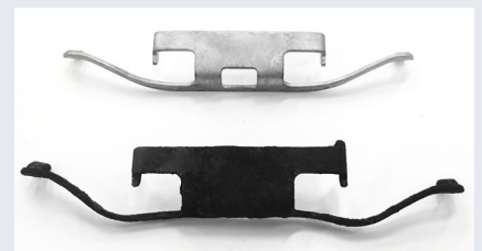
Top: New brake caliper spring Bottom: Brake caliper spring with considerably reduced clamping force after approximately 6 years of use, including extended periods of non-use.
